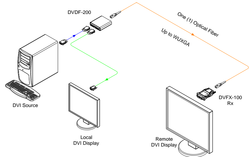
Figure 1 – Connection Diagram of DVDF-200
